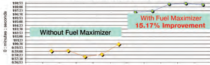
SAE J1321 Fuel Consumption Test Results Engine Tested Cummins N14 with #2 Sinclair Diesel Stationary Test 1oz to 23 gallons of fuel
